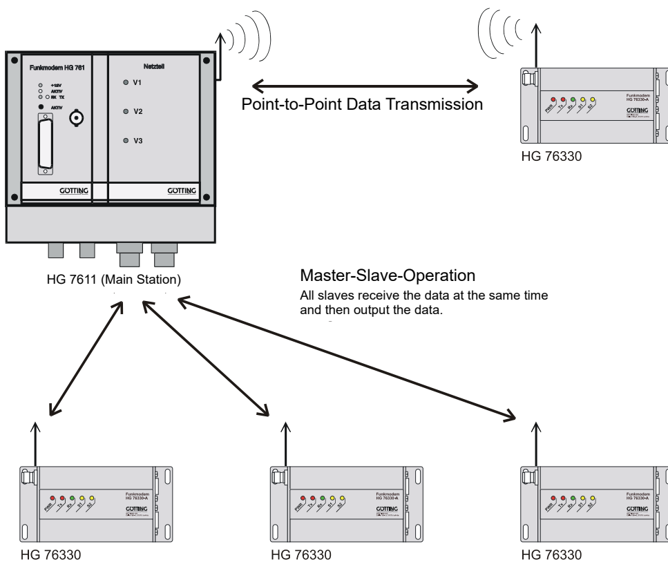
Figure 18 Simple Point to Point data transmission and bus topology with Master- Slave Operation
