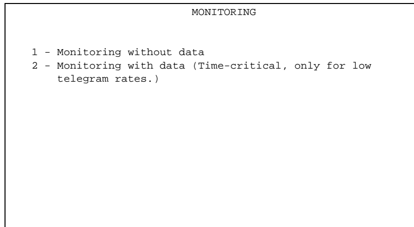
Figure 12 Screenshot: Monitoring
