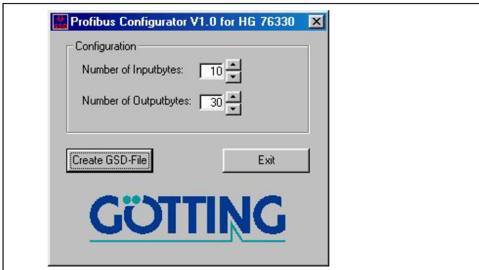
Figure 16 Screenshot
